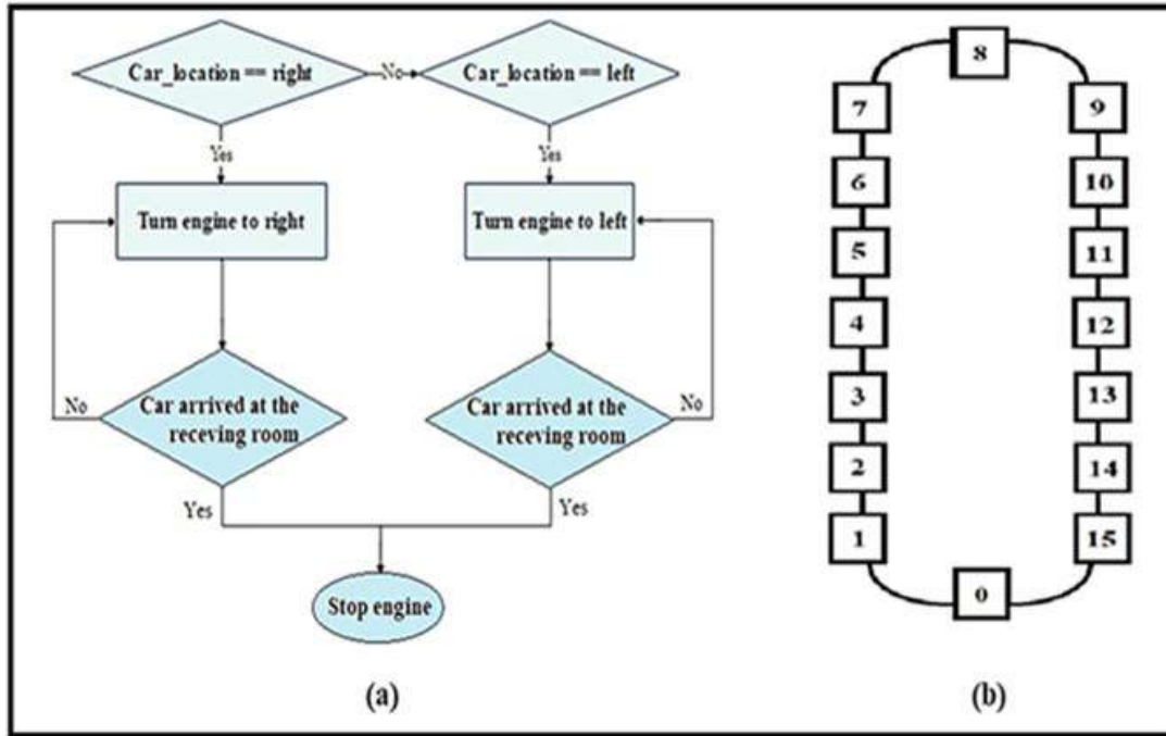
Figure 5. Shortest Path Detection
